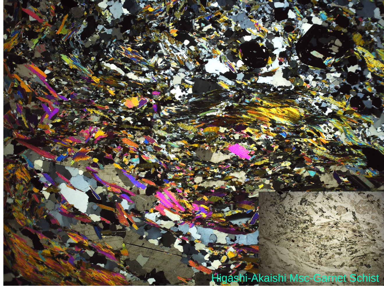
Kirishima Py-Andesite
